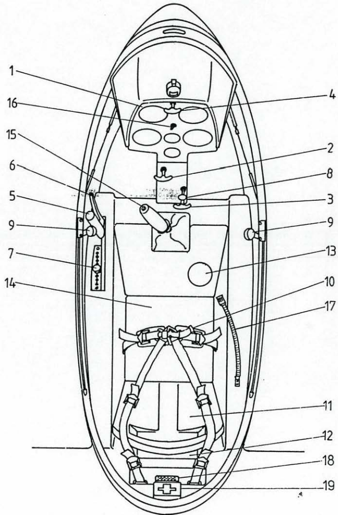
Cockpit devices Fig. 7 - 1
