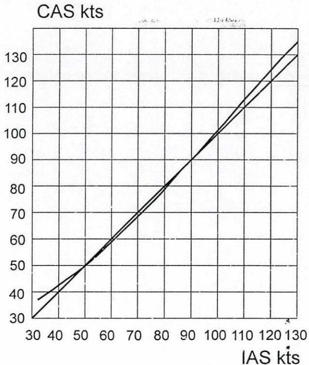
Airspeed indicator system calibration
